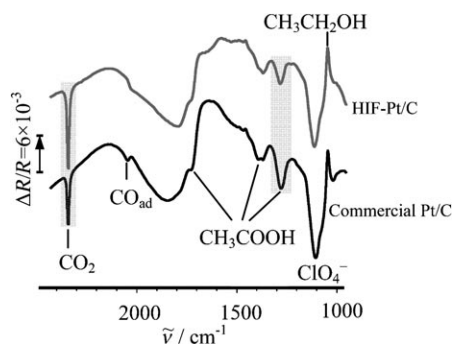
Figure 5. In situ FTIR spectra of ethanol oxidation on HIF-Pt/C and commercial Pt/C at 0.60 V in a mixture of 0.1 M ethanol and 0.1 M HClO 4 . Reference potential was –0.25 V.
